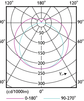
Light Distribution Diagram - MAS LEDtube 1500mm UO 20W 830 T8 EELC
